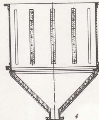
STEEL LEAD LINED VERTICAL CONE BOTTOM TANK SHOWING BRICK LINING IN CONE PORTION TO RESIST ABRASION . NOTE STRAPPING IN SHELL.
