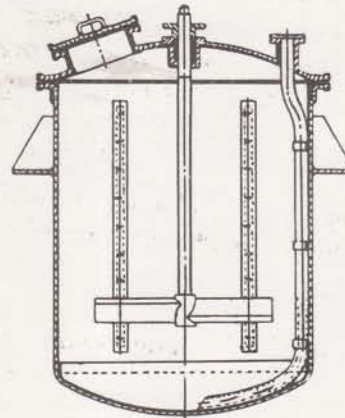
STEEL LEAD LINED VERTICAL DISHED BOTTOM TANK SHOWING STUFFING BOX LEAD COVERED AGITATOR & BLOW PIPE.
