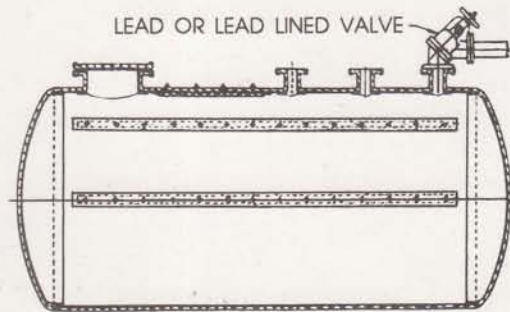
STEEL LEAD LINED HORIZONTAL TANK WITH DISHED HEADS & SUPPORTING LEAD LINING
