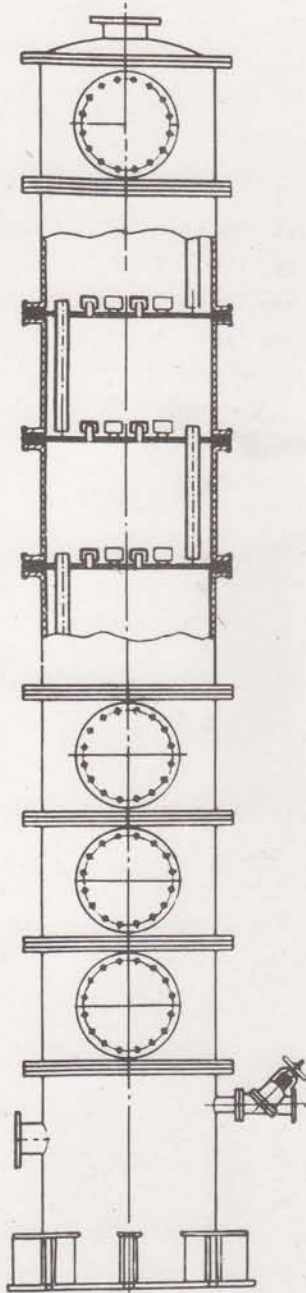
LEADLINED STEEL SECTIONAL TOWER SHOWING ANTIMONIAL LEAD TRAYS & BUBBLE CAPS.
